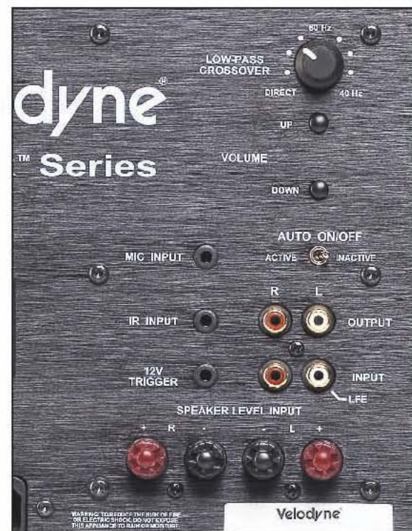
▲ Velodyne SPL-1200R
